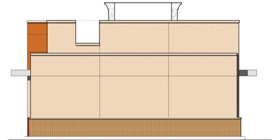
A1 REAR ELEVATION
