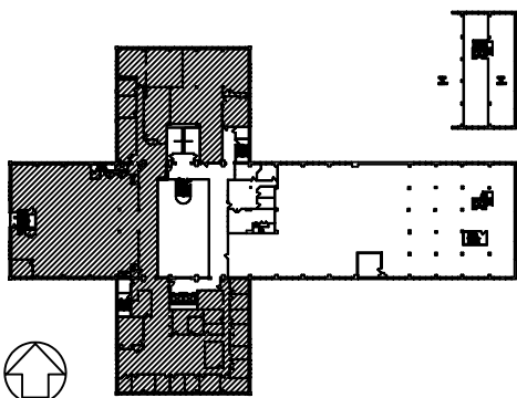
PLAN NORTH
