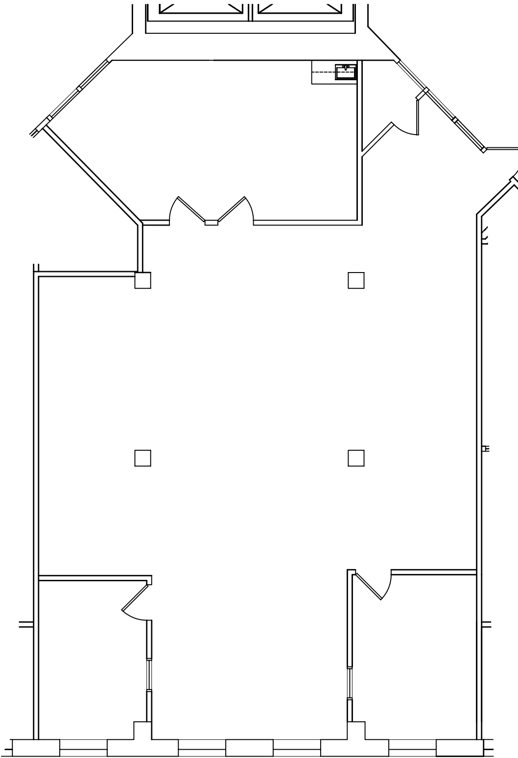
KEY PLAN - 1ST FLOOR
