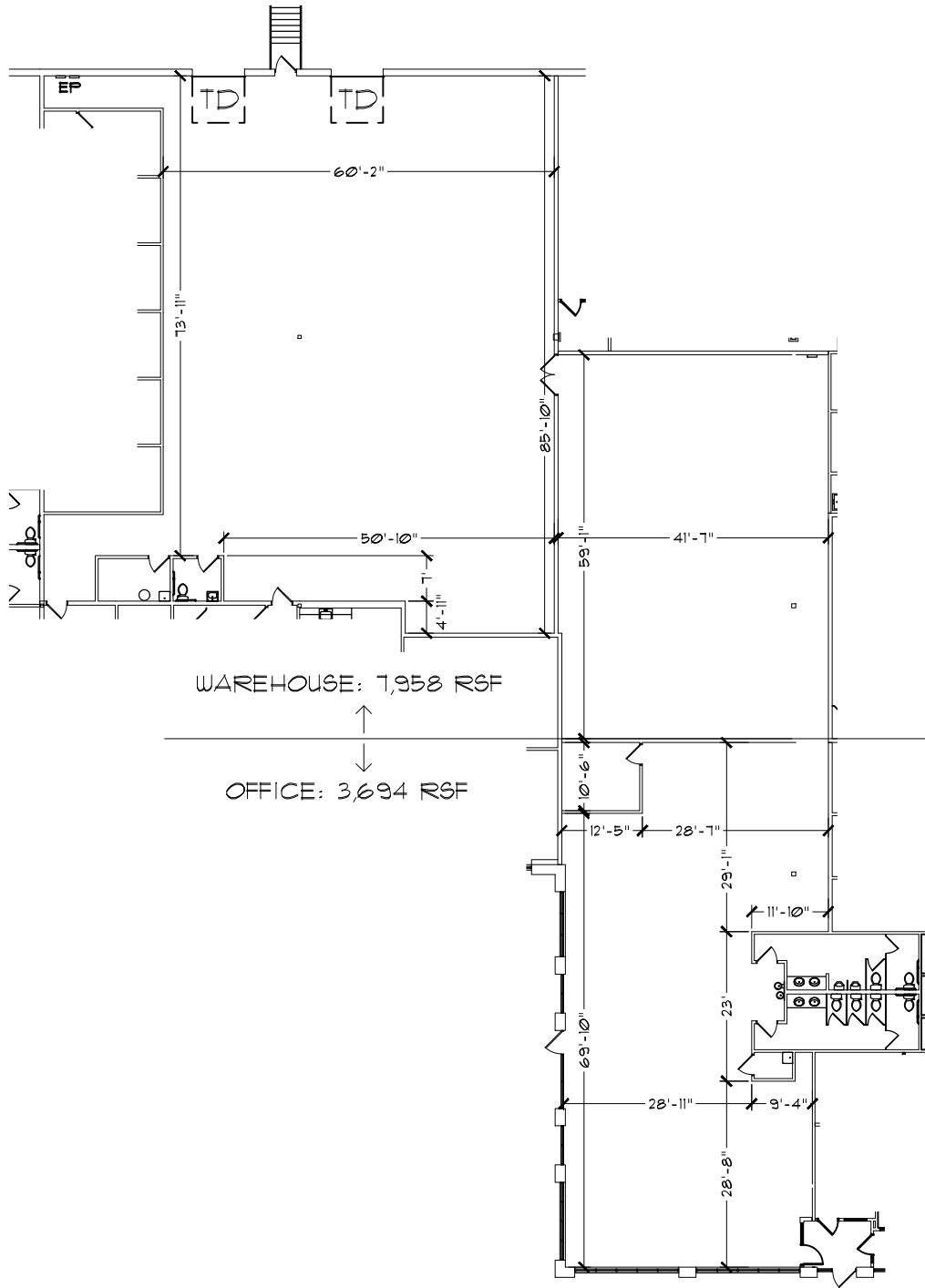
KEY PLAN - 1ST FLOOR
