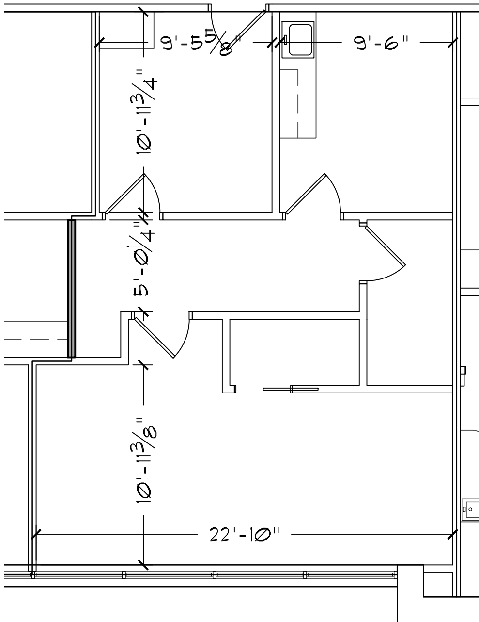
KEY PLAN - 1ST FLOOR
